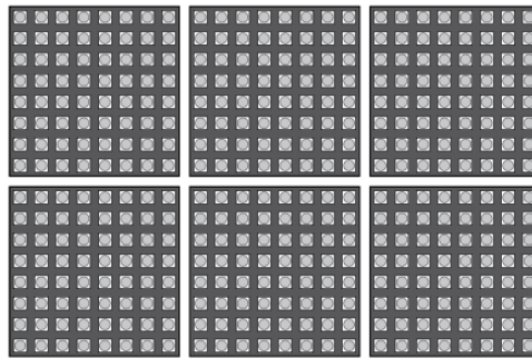
Tiled Matrices
