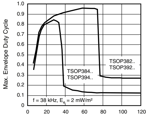
20754-2 Burst Length (number of cycles/burst) Fig. 9 - Max. Envelope Duty Cycle vs. Burst Length
