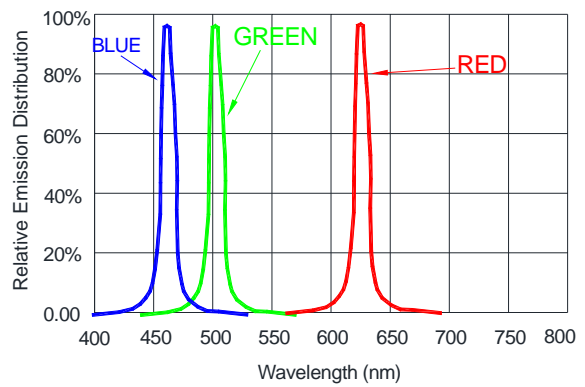
Wavelength Characteristics
