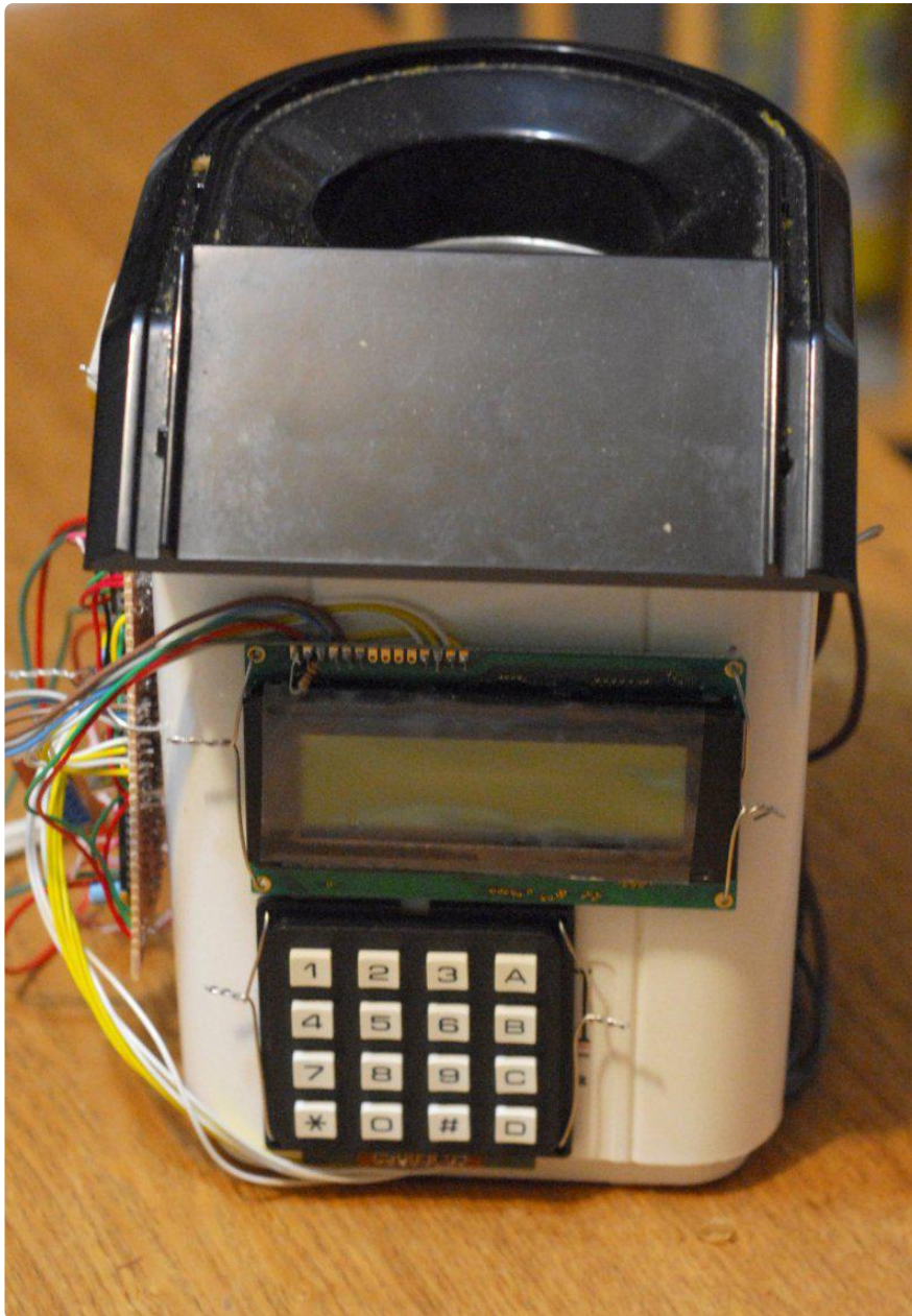
Terran's PI controlled coffee roaster (https://adafru.it/aLm)
