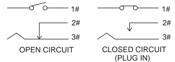
SCHEMATIC
