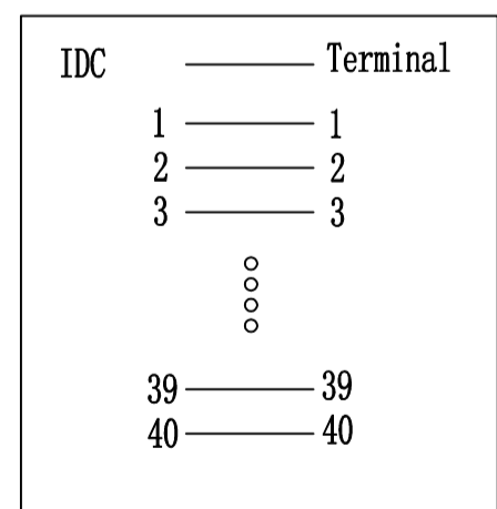
Pin assignment
