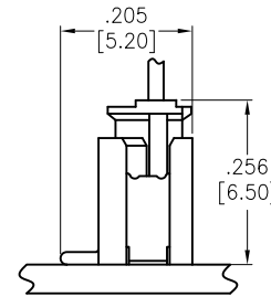
ASSEMBLY VIEW
