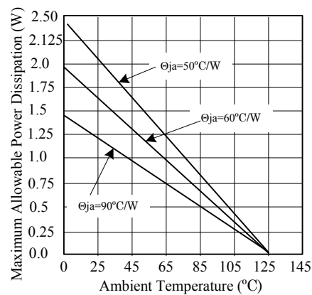
TO-252 Power Dissipation Still Air 20z Cu on top Plane
