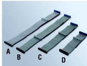
A. P/N 1701400973 HDD cable, ATA 66/100, 62 cm + 35 cm B. P/N 1701400972 HDD cable, ATA 66/100, 82 cm + 15 cm C. P/N 1701400652 HDD cable, ATA 66/100, 45 cm + 20 cm D. P/N 1701400452 HDD cable, ATA 66/100, 45 cm
