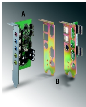
A. P/N PCA-AUDIO-00A1 Audio extension module (AC-97) provides Line-in, MIC-in, Aux-in, Line-out, Speaker-out, CD-in and Buzzer-in from CPU card
