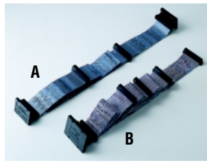
A. P/N 1701680670 68-pin SCSI LVDS cable, with 2 male connectors and terminators at both ends, 67 cm
