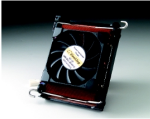
P/N 1759252100 CPU cooler for Pentium® 4 up to 2.53 GHz, for 1U chassis
