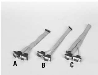
A. P/N 1701200180 Cable Flat cable 18 cm IDC 20P 2.0 mm/ 2 COM PCM-9576 use
