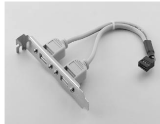
P/N 1700100170 USB Cable adaptor 17.5 cm 2CH w/guard hole No. 10P
