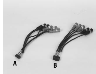
A. P/N 1700160160 Audio cable for PCM-5820/L 16-pin 16 cm (2.0 mm)
