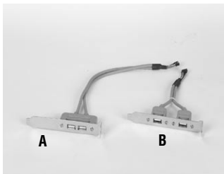
A. P/N 1703100260 Wire 10P 26 cm IDE 2.0 mm For USB 2 port 1.9"
