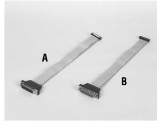
A. P/N 1700260250 Cable ASSY LPT port 25 cm 25P to 26P 2.0 mm
