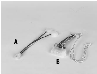
A. P/N 170304015K Wire Big 4P*2/4200-H-4P 15 cm
