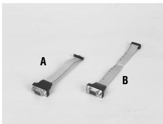
A. P/N 1701160101 Cable ASS'Y VGA 10 cm D-SUB 15P to 16P 2.0 mm
