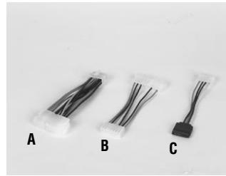
A. P/N 1700000265 Wire ATX-20P (M)/12P (F) 10 cm PCM-9581
