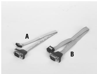
A. P/N 1700100250 Cable ASS'Y COM port 25 cm D-SUB 9P to 10P 2.0 mm
