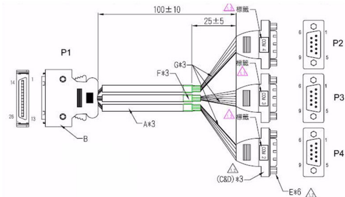
Figure 2.14 COM2~4 cable
