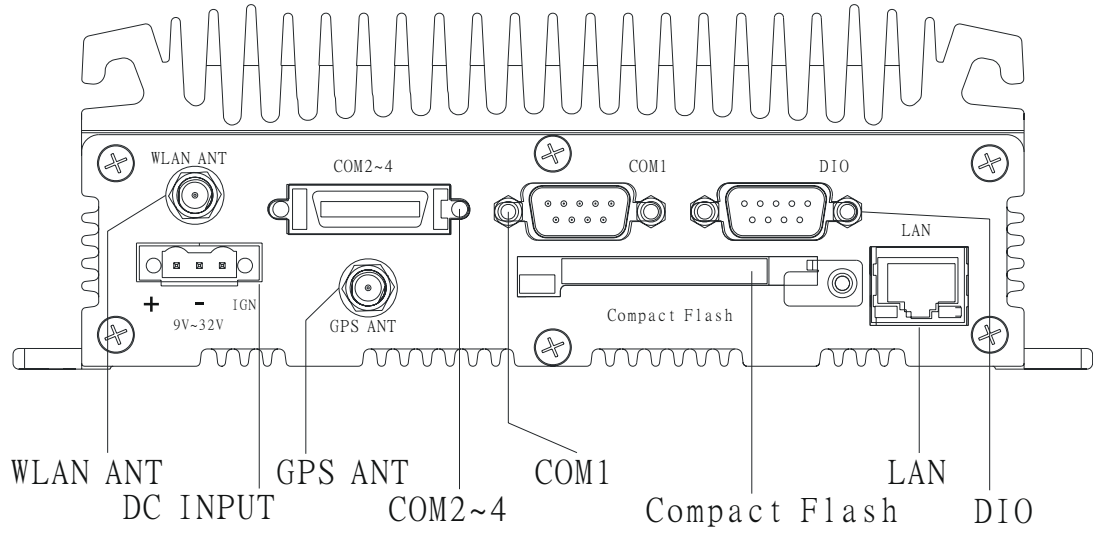
Figure 2.4 ARK-1388V Rear I/O Panel
