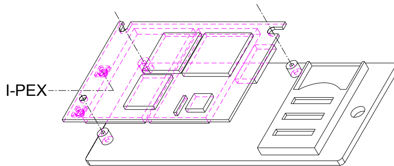
Figure 5.9 install Siemens module on AMO board
