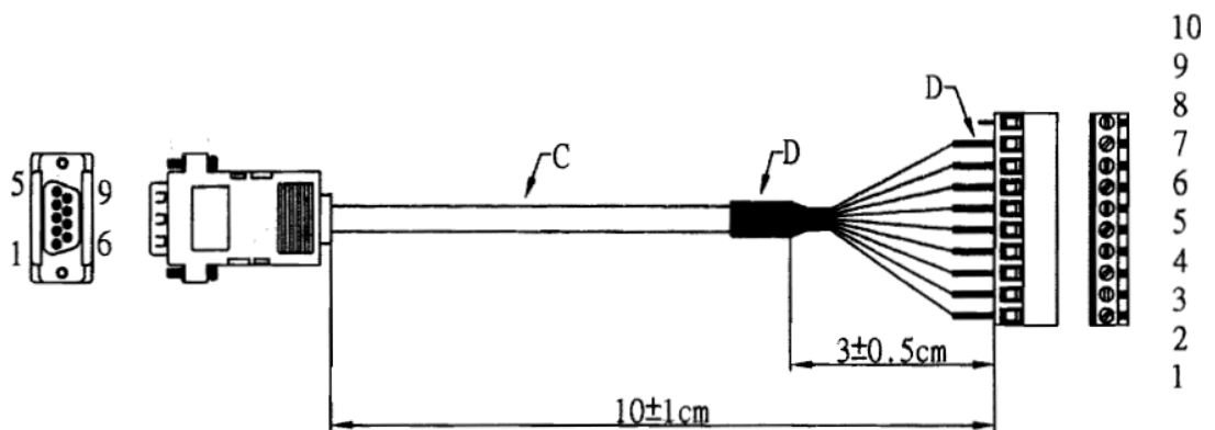
Figure 2.12 DIO cable
