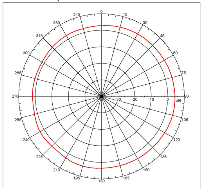
Far-field amplitude of 1206TEST-1 2.4GHz-H.nsi
