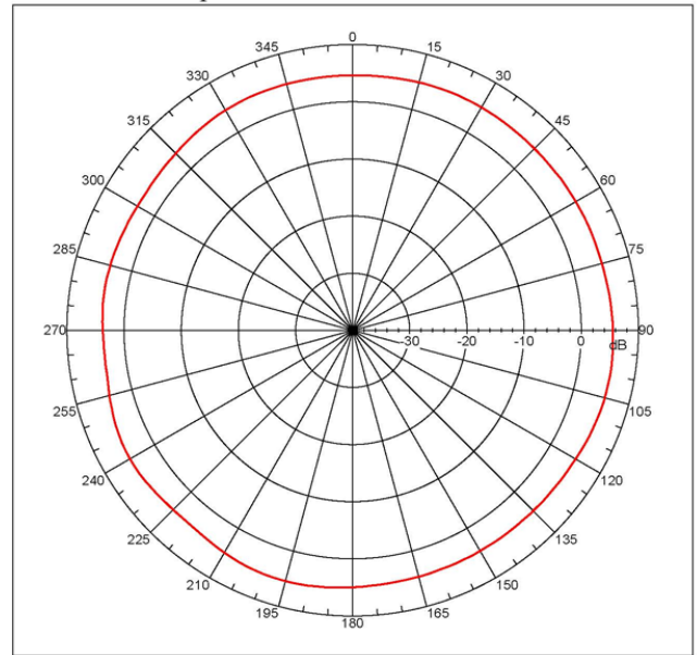
Far-field amplitude of 1206TEST-1 2.4GHz-H.nsi
