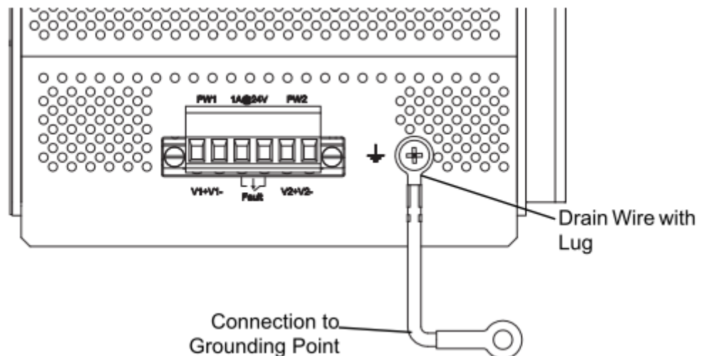
Figure 1-16. Grounding Connection
