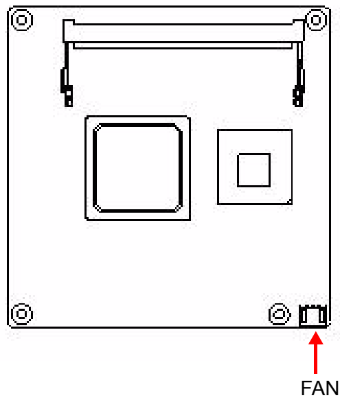
Figure 2.1 Board Layout (component side)
