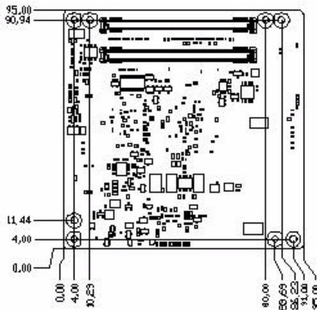
Figure 2.4 Board Dimension (Solder side)
