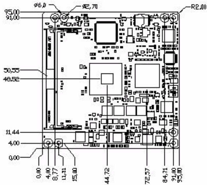
Figure 2.3 Board Dimension (Component side)
