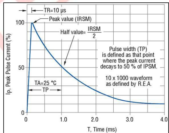
Figure 4- Pulse Waveform
