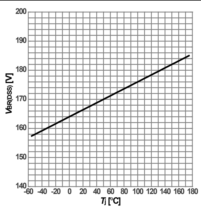
Diagram 11: Breakdown Voltage Variation vs. Temperature
