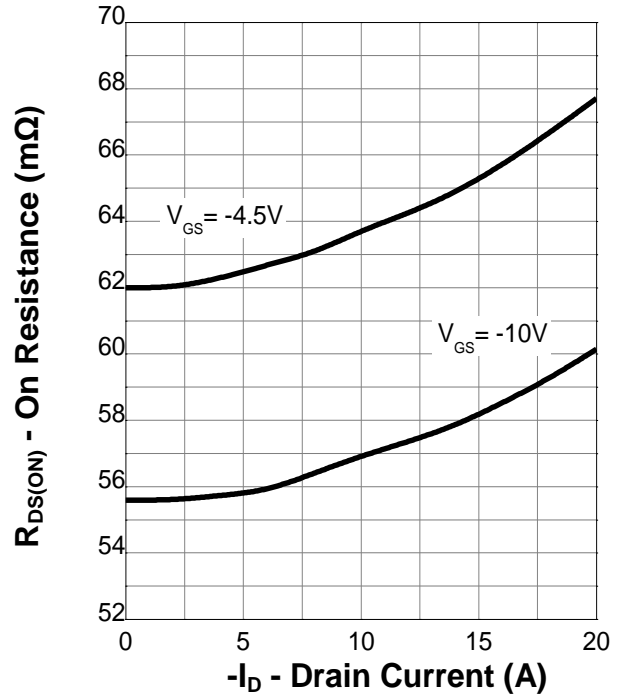
On Resistance
