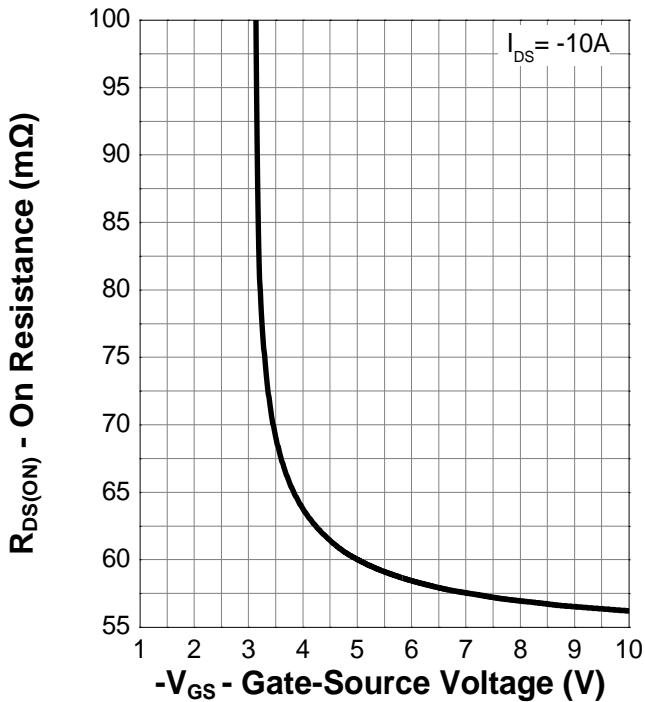
Transfer Characteristics
