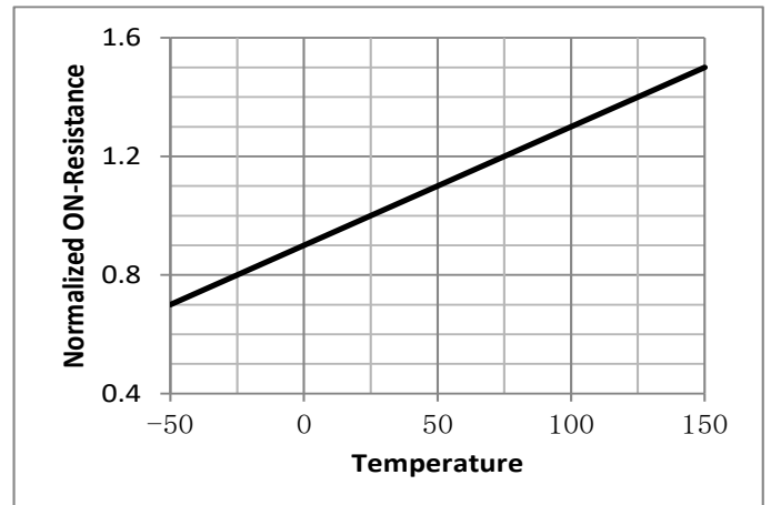
Fig.6 On-Resistance V.S Junction Temperature
