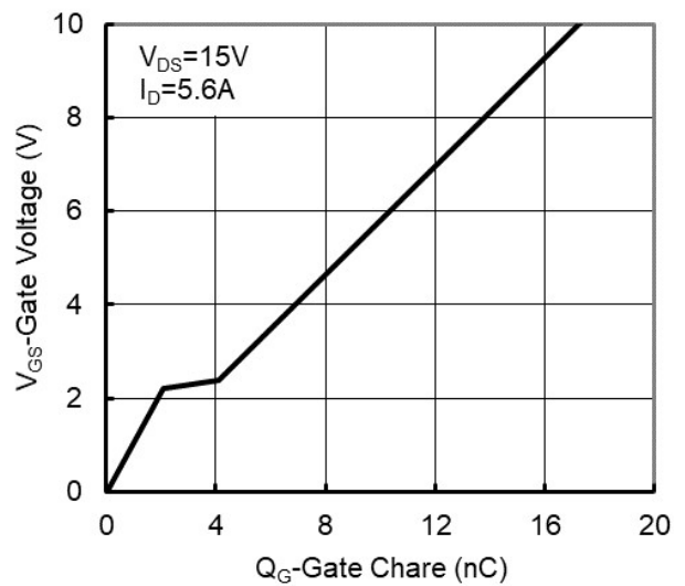
Figure6. Gate Charge
