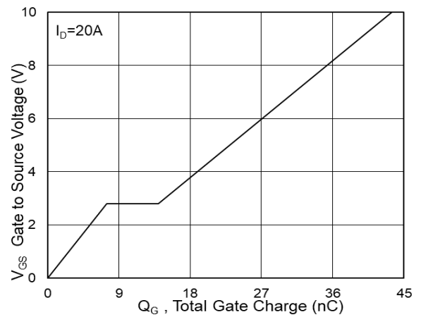
Fig.4 Gate-Charge Characteristics
