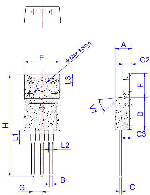
TO-220F
