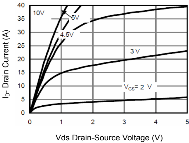
Figure 3 Output Characteristics
