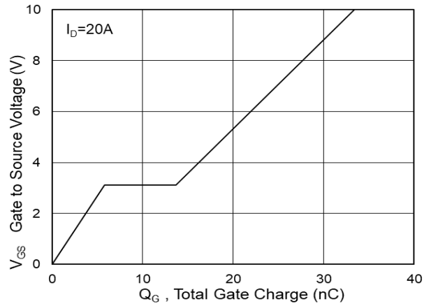
Fig.4 Gate-Charge Characteristics
