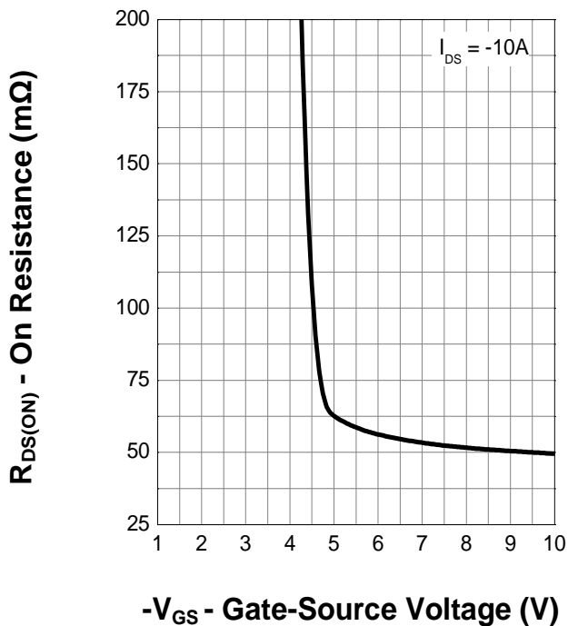
Transfer Characteristics
