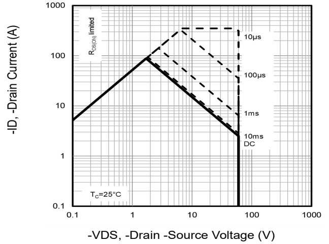
Fig8. Maximum Safe Operating Area
