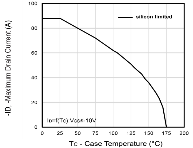
Fig12. Maximum Drain Current Vs. Case Temperature
