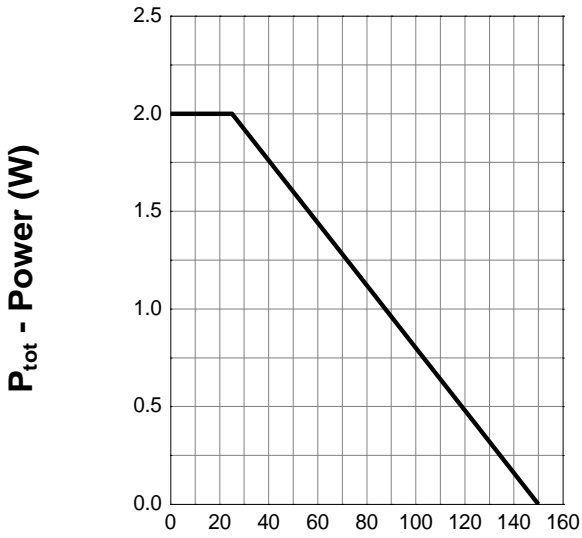
T_{mp} – Mounting Point Temp. (°C)
