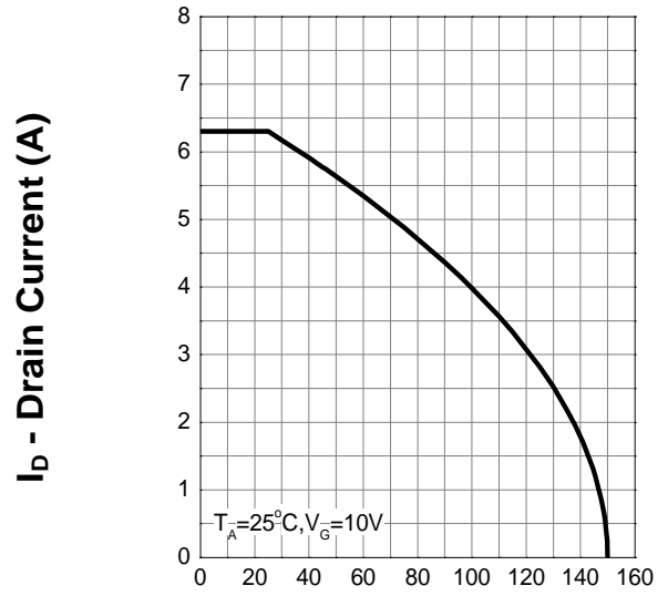
T_{mp} – Mounting Point Temp. (°C)
