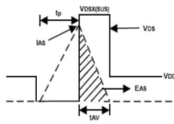
Fig14. Unclamped Inductive Test Circuit and waveforms
