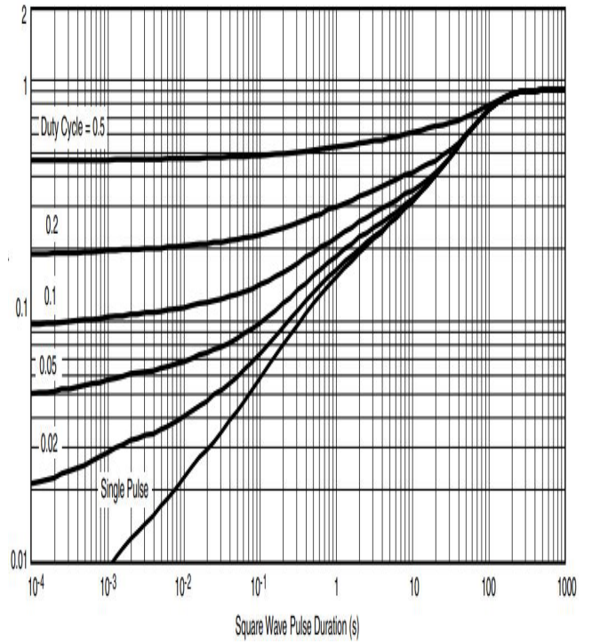
Fig8. Normalized transient thermal impedance
