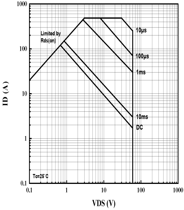
Fig7. Safe Operating Area
