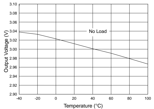
Fig. 21 AIC1642-30 Output Voltage vs. Temperature
