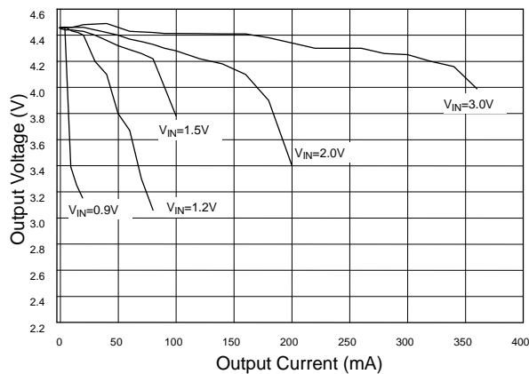
Fig. 44 AIC1642-45 Load Regulation (L=100µH)
