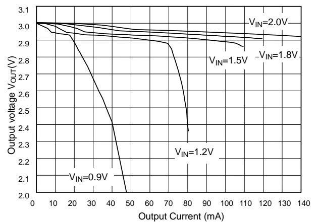
Fig. 15 AIC1642-30 Load Regulation (L=100μH, CD54)
