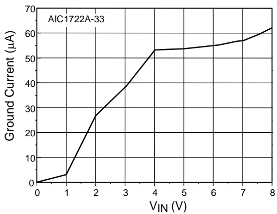
Fig. 11 Ground Current vs. V_{IN}
