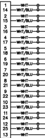
25 POSITION
