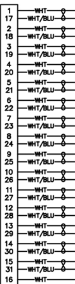
31 POSITION
