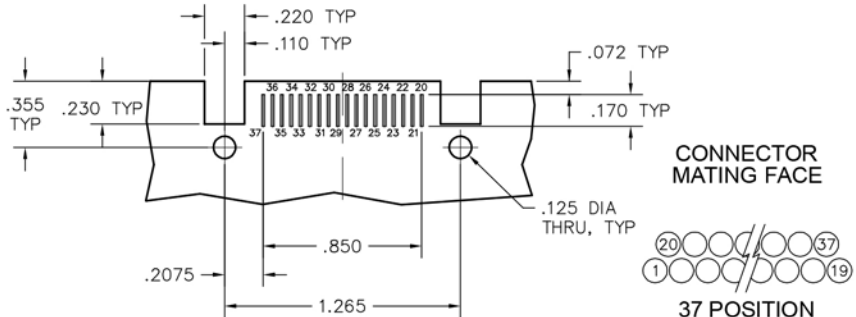
RECEPTACLE PC BOARD LAYOUT COMPONENT SIDE
