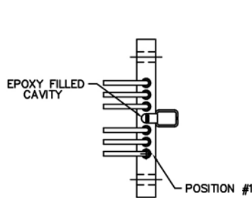
TERMINATION VIEW
