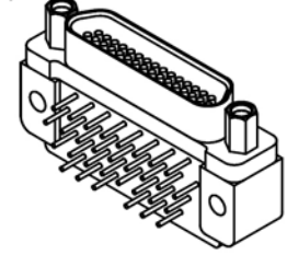
MK-2S2-031-445-220S (RCPT)
