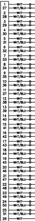
51 POSITION 2 rows
