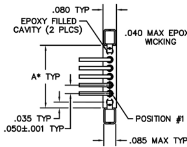
TERMINATION VIEW
