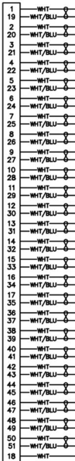
51 POSITION 3 rows
