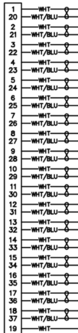
37 POSITION
