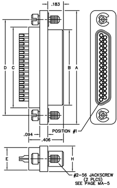
PLUG
