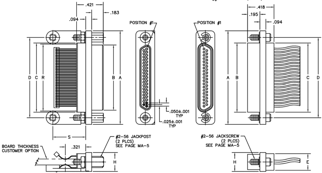
PLUG
