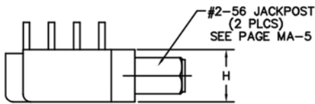
PLUG
