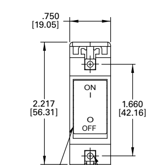
OPTIONAL GUARD (SEE DETAIL "A") 6-32 THD. MOUNTING M3 ISO THD. OPTIONAL
