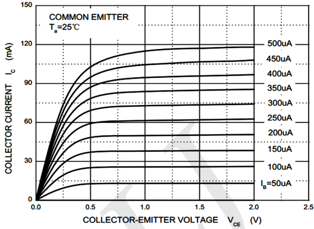
Static Characteristic
