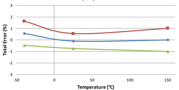
Total Error at I_{PR(max)} vs. Temperature
