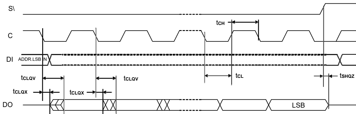
Figure 13. Output Timing
