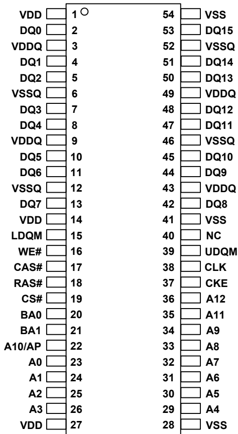
Figure 1.A. Pin Assignment (Top View)
