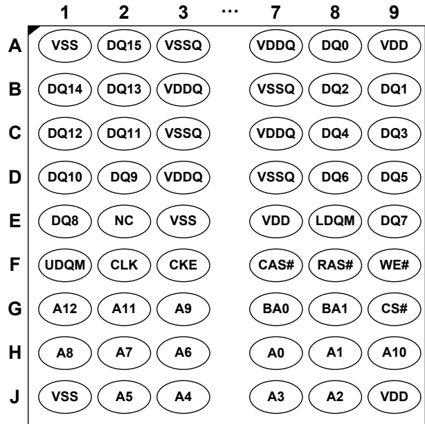
Figure 1.B. Ball Assignment (Top View)
