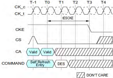
Figure 24. tESCKE Timing
