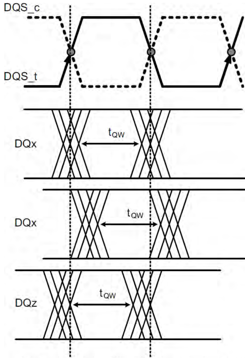
Figure 33. Read data timing t_{QW} valid window defined per DQ signal
