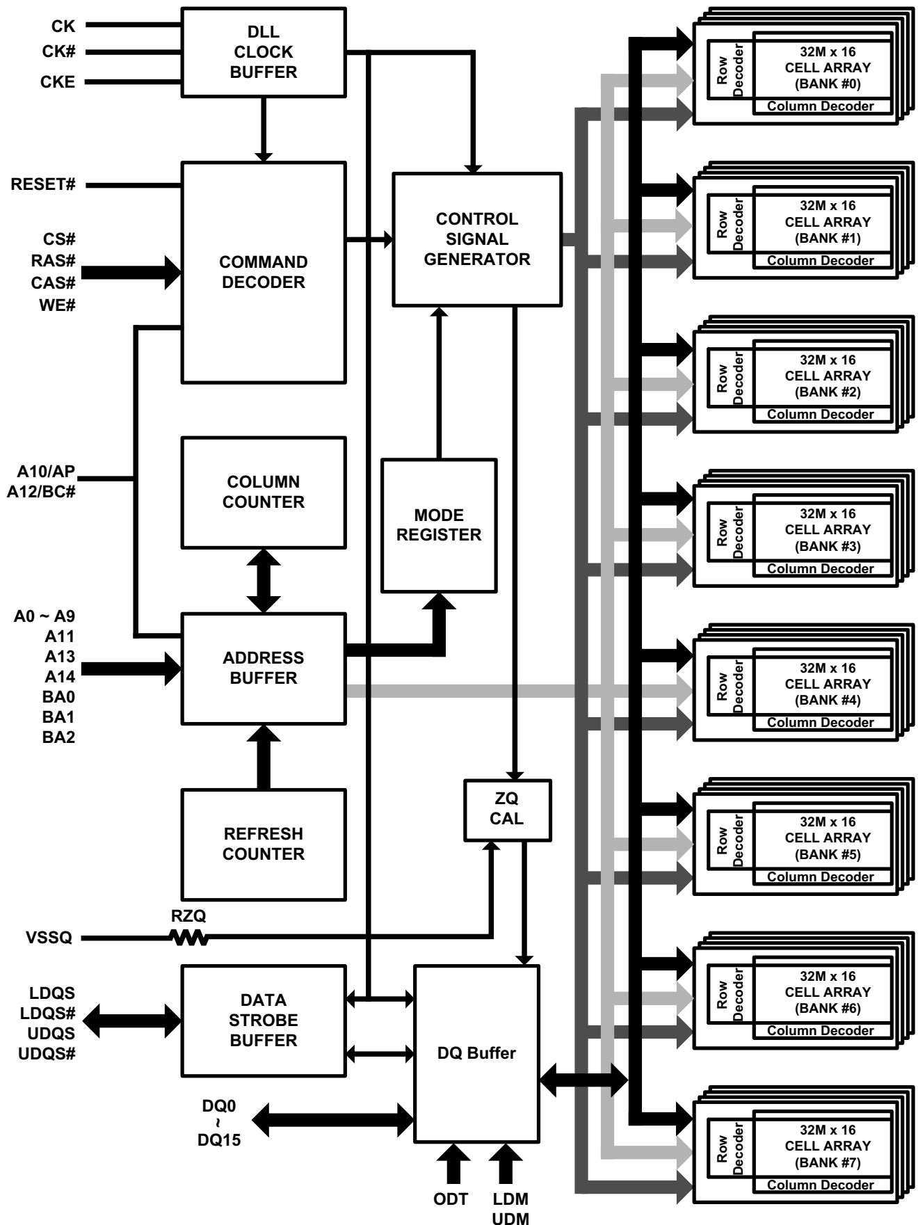
Figure 2. Block Diagram
