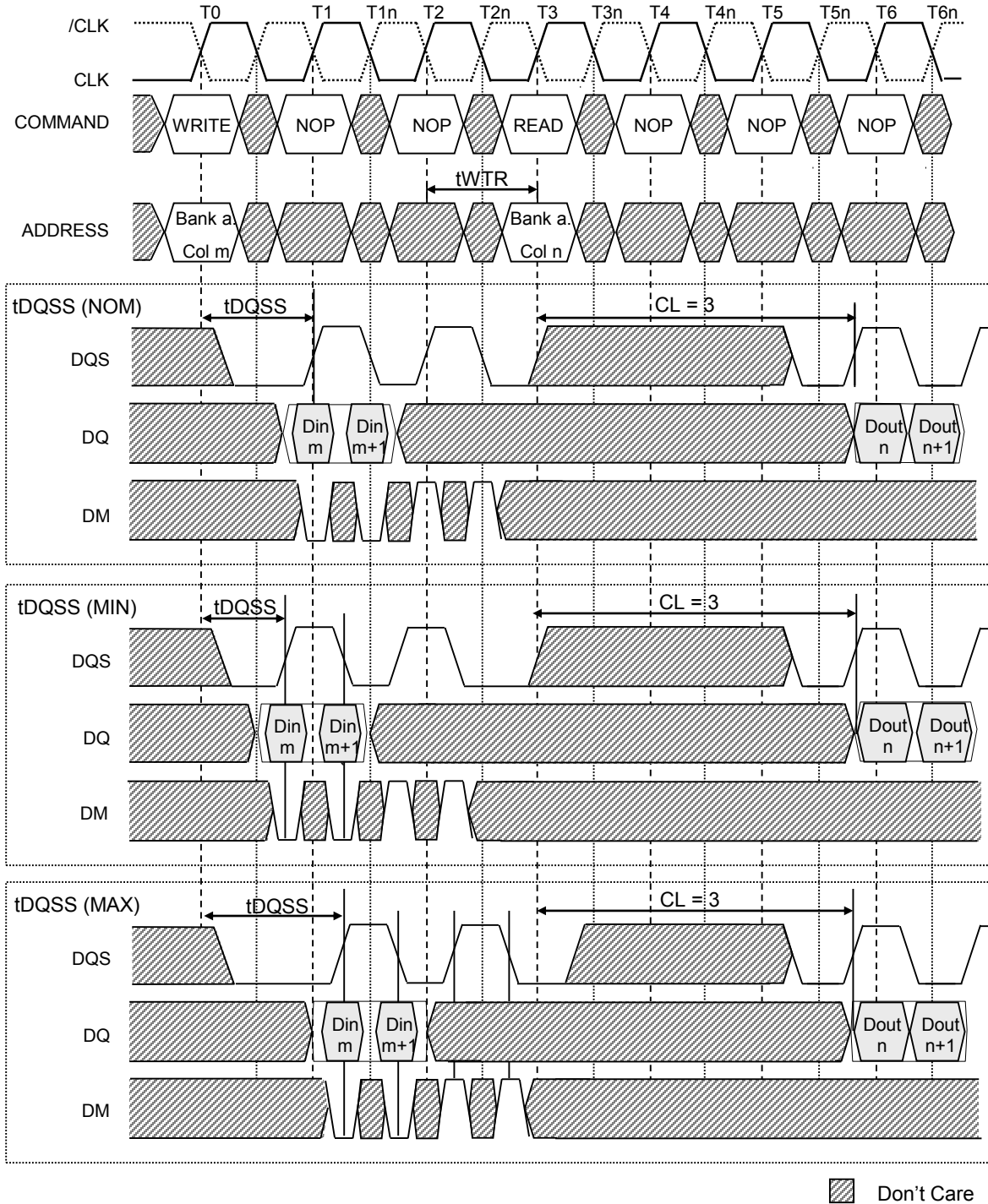
Figure 20: WRITE-to-READ – Interrupting
