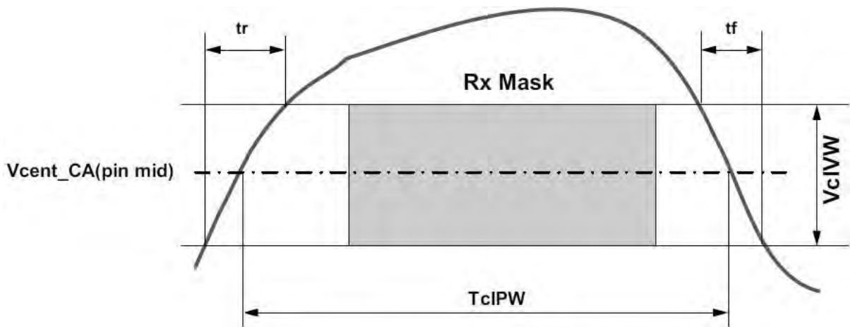
Figure 30. CA TcIPW and SRIN_cIVW definition (for each input pulse)
