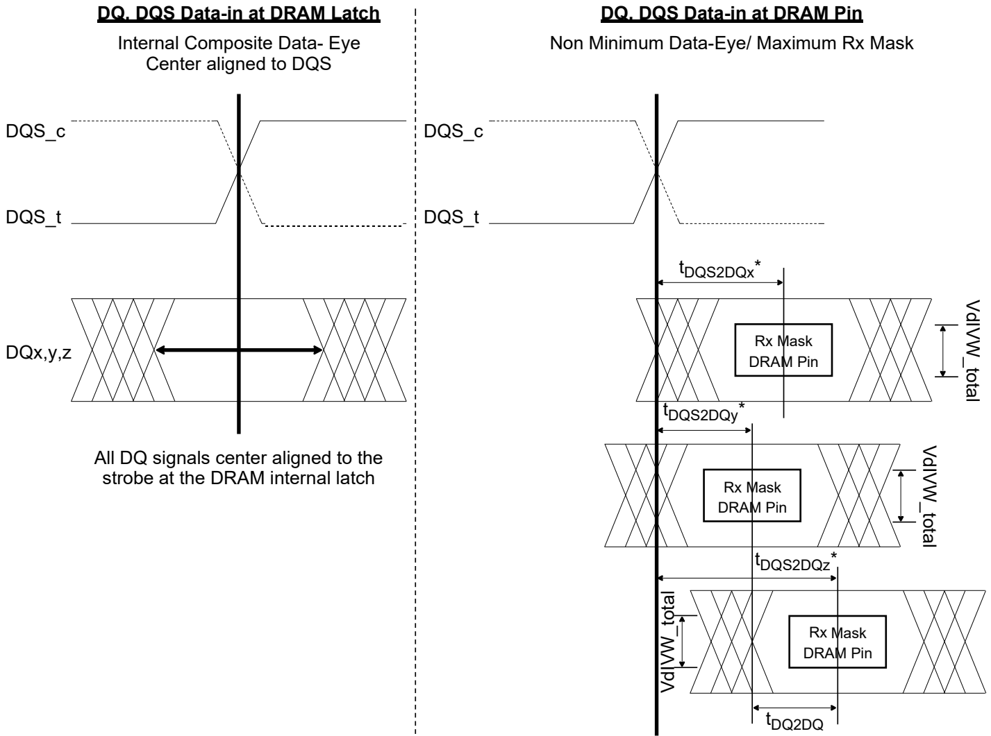
Figure 36. DQ to DQS t_{DQS2DQ} & t_{DQDQ} Timings at the DRAM pins referenced from the internal latch
