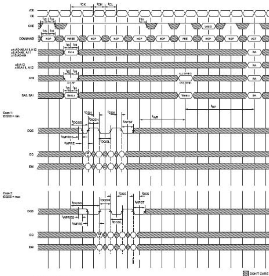
Figure 45 - WRITE - WITHOUT AUTO PRECHARGE
