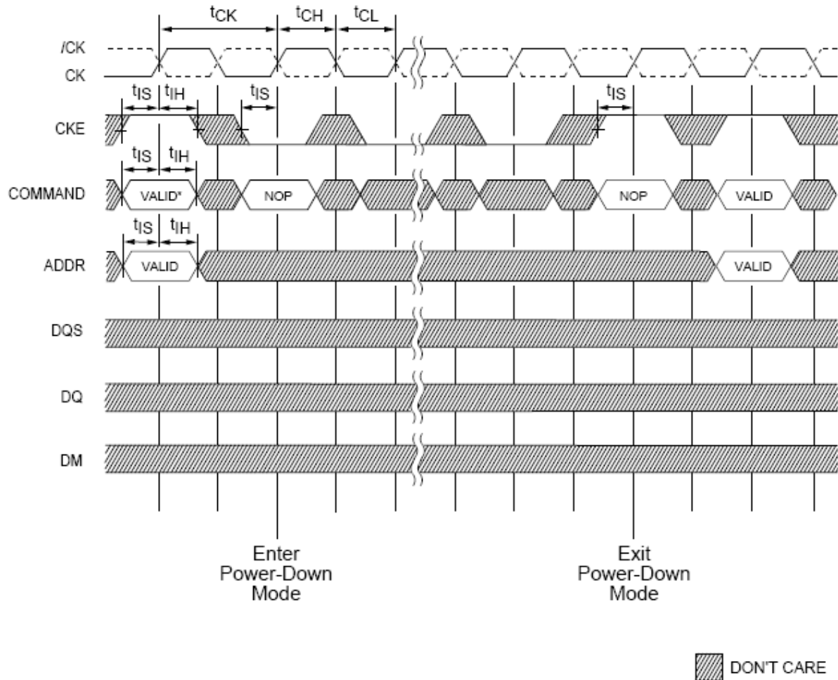
Figure 39 - POWER-DOWN MODE
