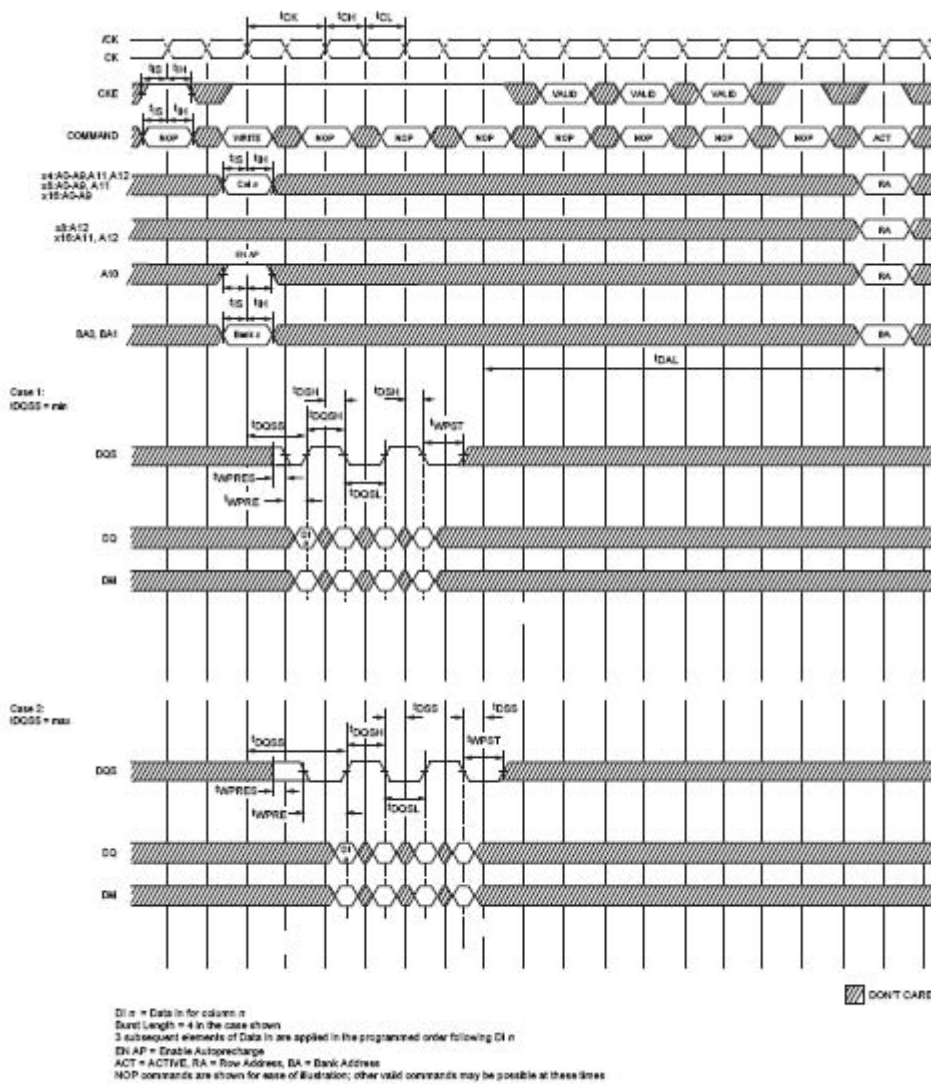
Figure 46 - WRITE - WITH AUTO PRECHARGE
