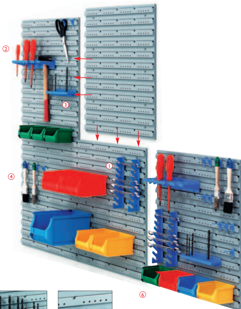
StorePlus Set »P« 17 Wall bracket + 1x wrench holder, 1x universal tool holder, 1x drill/bit holder, 4x hook 40, 6x hook 30 and 4x storage bin »ProfiPlus« size 1 (without tools)
