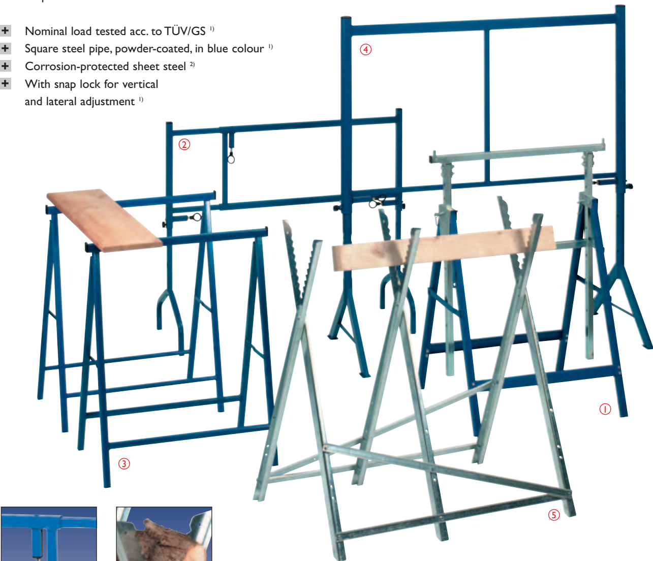
Snap lock for width/height adjustment (art. no. 430016 and 430013)
