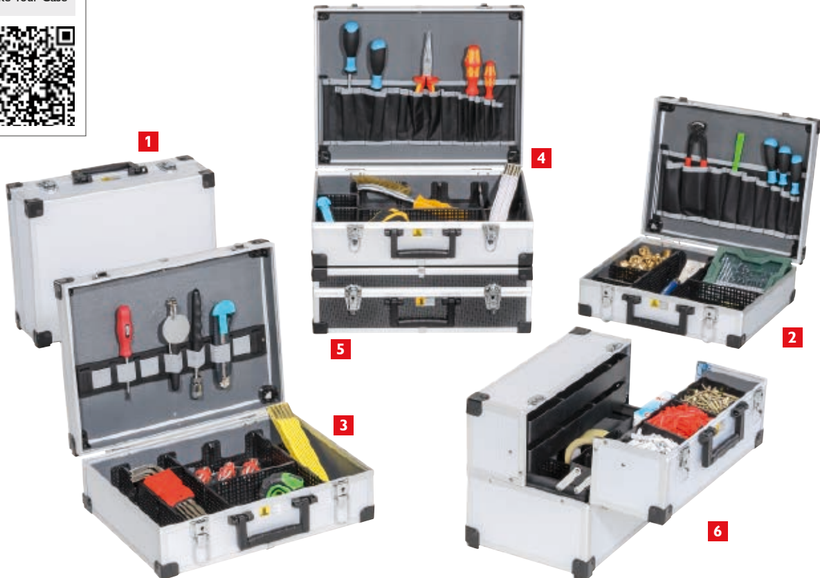
Arretierbare Kunststoff-Trennsteg in Schwalbenschwanzführung Plastic slide-in dividers in dovetailed guides for neat compartments
