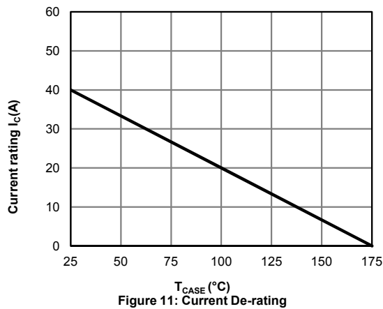
Figure 11: Current De-rating
