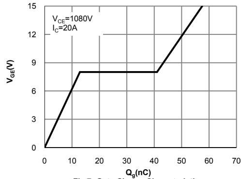
Fig 7: Gate-Charge Characteristics
