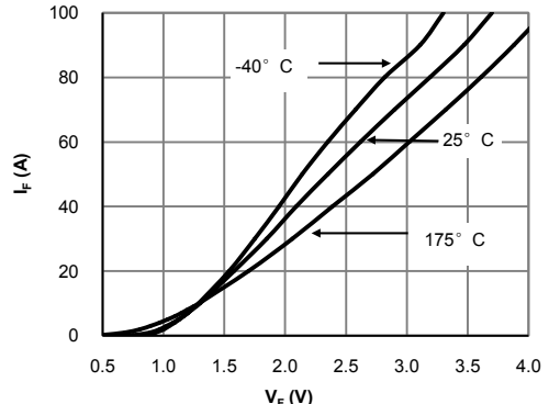
Fig 4: Diode Characteristic
