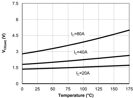
Fig 5: Collector-Emitter Saturation Voltage vs. Junction Temperature
