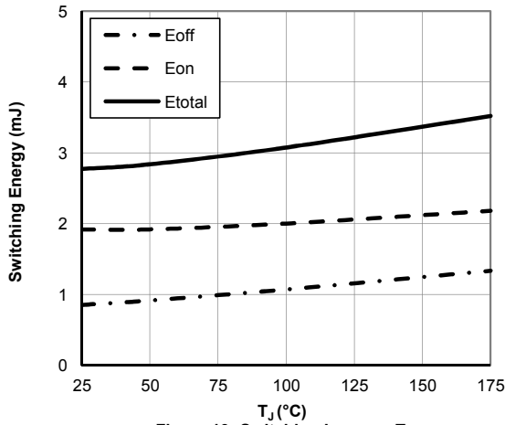
Figure 19: Switching Loss vs. T_j ( V_{GE}=15\text{V} , V_{CE}=400\text{V} , I_c=50\text{A} , R_g=6\Omega )
