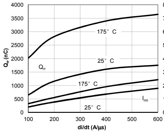
Figure 23: Diode Reverse Recovery Charge and Peak Current vs. di/dt ( V_{GE}=15V , V_{CE}=400V , I_F=60A )
