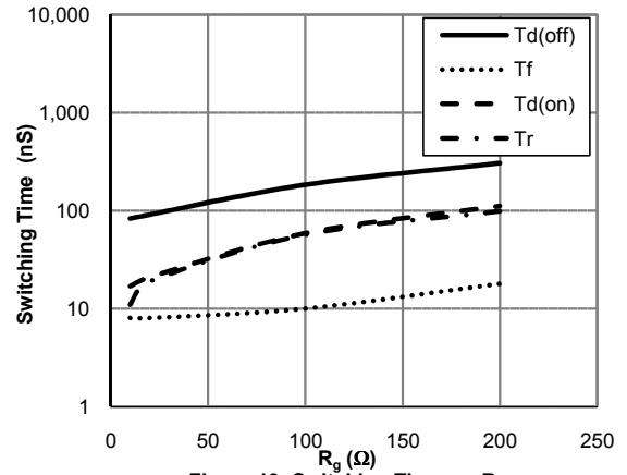
Figure 13: Switching Time vs. R_g ( T_j=150^\circ\text{C}, V_{GE}=15\text{V}, V_{CE}=400\text{V}, I_c=15\text{A} )
